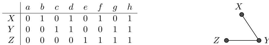
Figure 2.3: Comparison of X, Y, Z \in \Gamma_{E(T_n)} .
