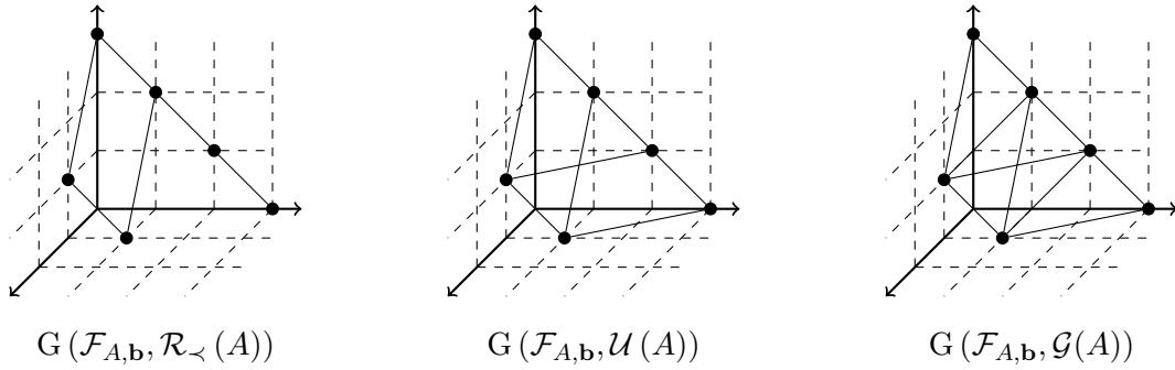
Figure 1: Different fiber graphs of the same underlying fiber.
