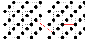
Figure 2: Different types of Graver moves of A_k .
