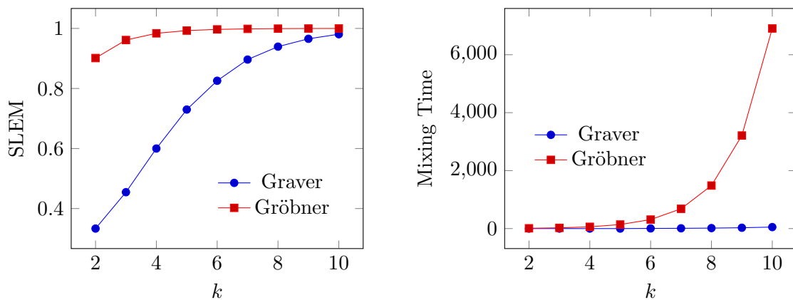
Figure 4: Plots of SLEM and mixing time of \mathcal{F}_{A_k, \mathbf{e}_{2k+1}} with respect to Graver and Gröbner moves.
