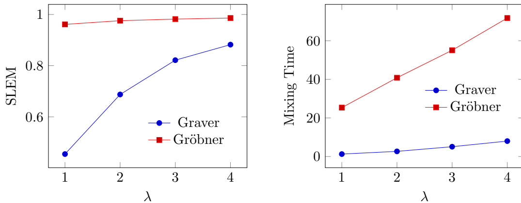
Figure 5: Plots of SLEM and mixing time of \mathcal{F}_{A_3, \lambda \cdot \mathbf{e}_7} with respect to Graver and Gröbner moves.
