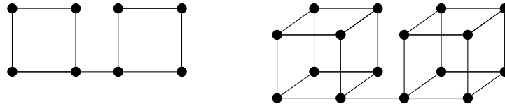
Figure 3: A sketch of \mathcal{B}_{\mathbf{e}_{2k+1}}(0) and \mathcal{B}_{\mathbf{e}_{2k+1}}(1) for k = 2 and k = 3 with respect to Gröbner moves.
