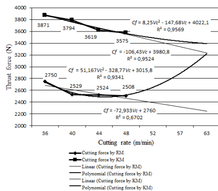
Fig. 4. Thrust force value change graph against increasing untested test parameters at 10%
