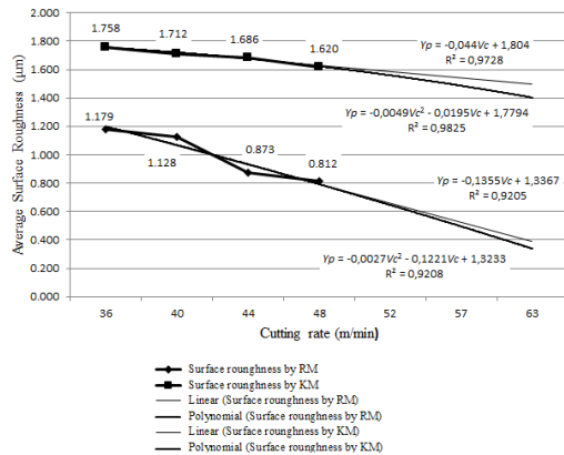
Fig. 6. Average surface roughness value change graph against increasing untested test parameters at 10%
