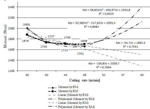
Fig. 5. Moment value change graph against increasing untested test parameters at 10%
