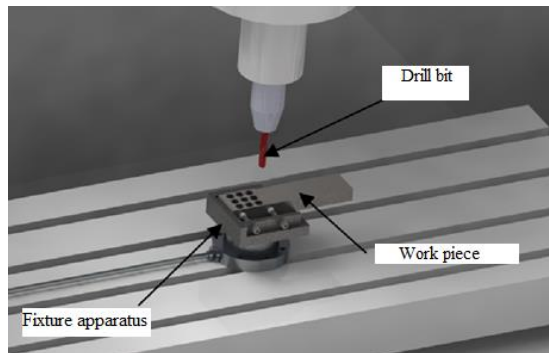
Fig. 2. Fixture apparatus
