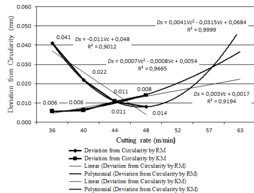
Fig. 8. Deviation from circularity value change graph against increasing untested test parameters at 10%
