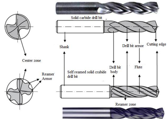
Fig. 3. Tool geometry of carbide drills (Özkul 2012)
