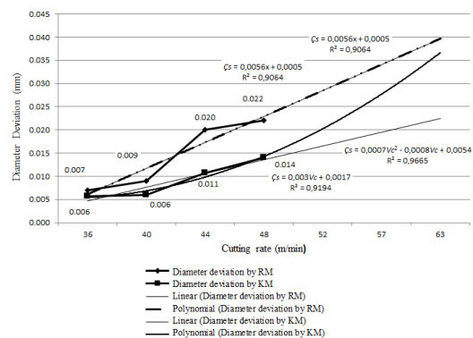
Fig. 7. Diameter dimension value change graph against increasing untested test parameters at 10%
