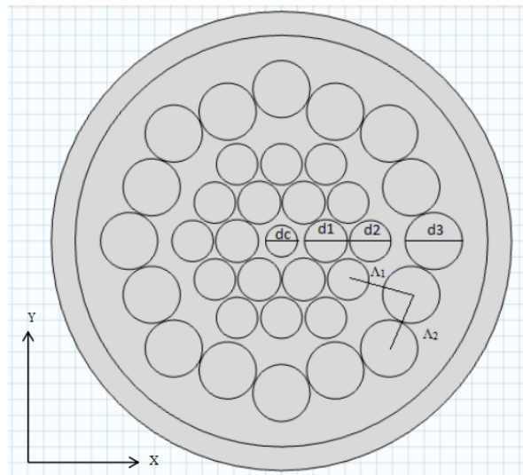
Fig. 1 Transverse Cross-sectional view of proposed structure
