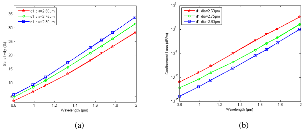
Fig. 5 (a) Relative sensitivity versus Wavelength and (b) Confinement loss versus Wavelength for d1=2.60 \mu\text{m} , d1=2.75 \mu\text{m} and d1=2.80 \mu\text{m} when dc=2.0 \mu\text{m} , d2=2.70 \mu\text{m} and d3=3.50 \mu\text{m} were optimized.
