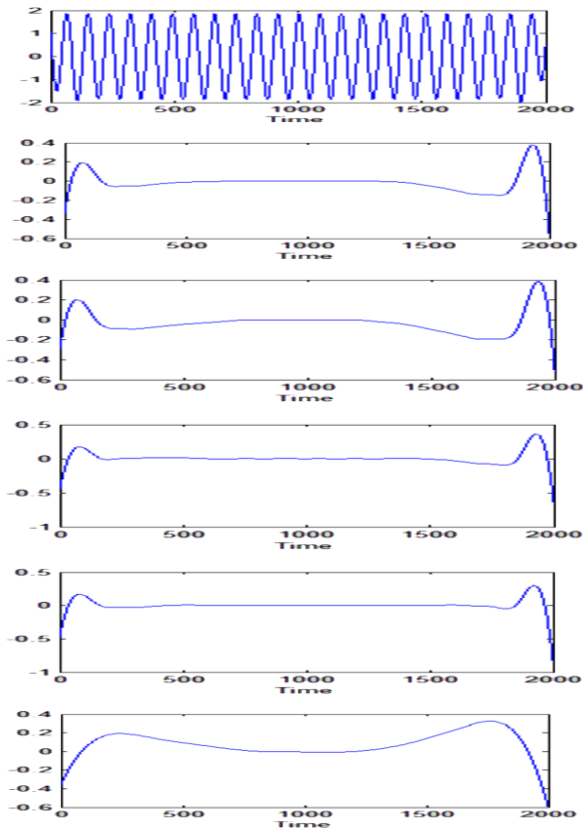
Fig. 5. IMF generate schematic drawing
