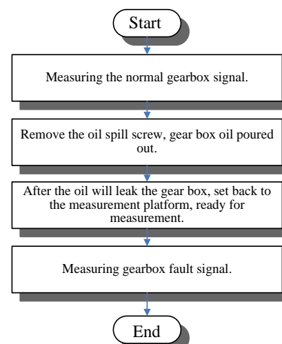
Fig. 1. Gear box oil leak fault gauging procedure.
