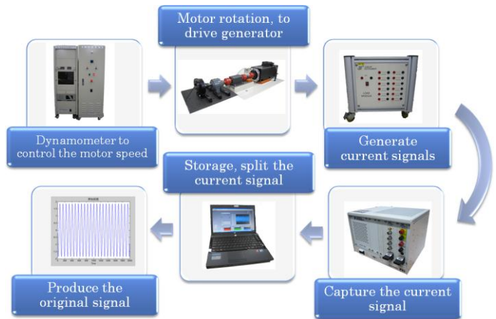
Fig. 2. Signal measurement process
