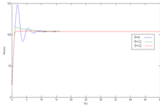
Figure 8. The output speed of the wind turbine rotor after designing the controller B=10 .
