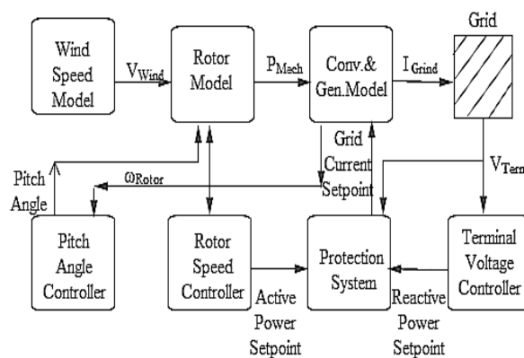
Figure 2. The turbine model and its controllers.
