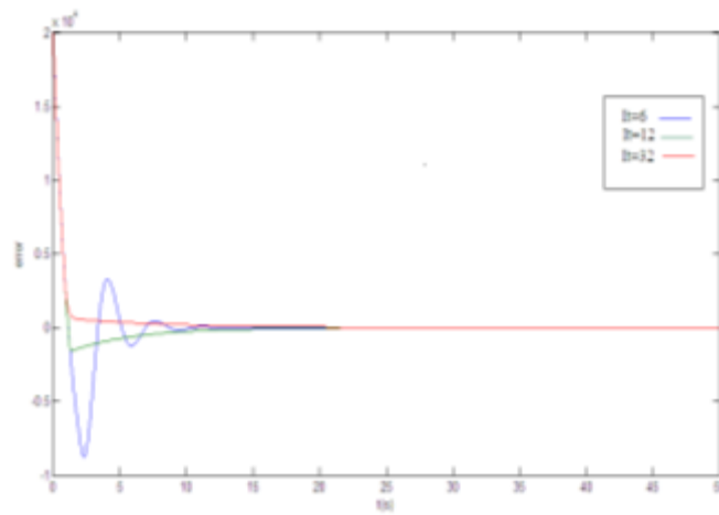
Figure 11. The (power) error of the wind turbine after designing the controller B=8.
