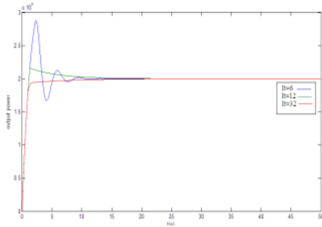
Figure 10. The output power of the wind turbine after designing the controller B=10.
