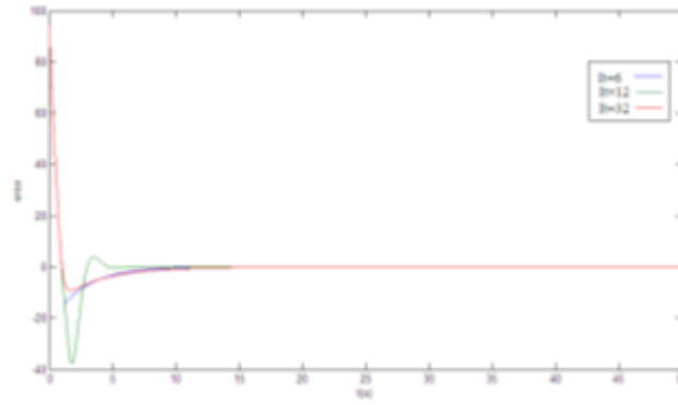
Figure 13. The (rotor speed) error of the wind turbine after designing the controller B=8 .
