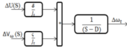
Figure 3. A block diagram of the linearized model of a wind turbine.
