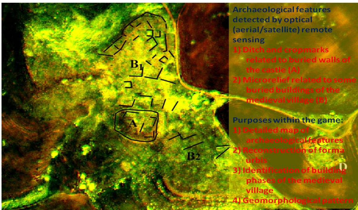
Figure 7. First approach: discovery of unknown archaeological features using VHR satellite data, details in [3].
