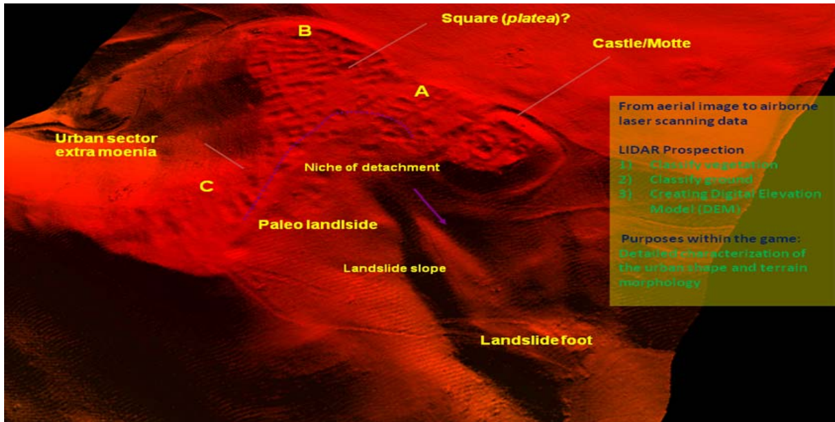
Figure 8. Identification of urban shape of the lost medieval village and palaeo-landslide in Monte Irsi [2].
